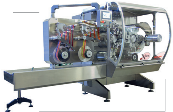
Wrapping machine for stock tablet and cubes at speed 1,000. Continuous motion. Size change from tablet to cube, and vice versa
