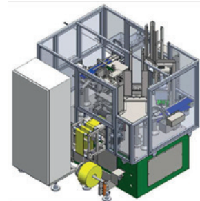
BTR 10 - Packaging machine. Bundling butter for tray and hood. Product: butter size hotel
