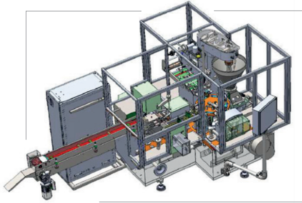
S23/C - Packaging machine. Wrapping, forming and cartoning machine. Products: soft cubes and cartoning
